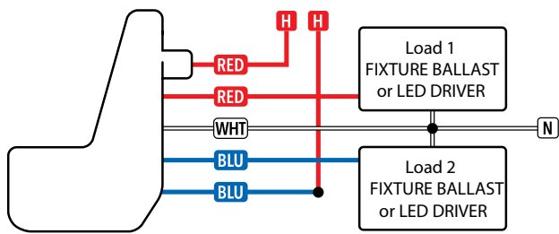
LINE VOLTAGE INTERCHANGEABLE LENS FIXTURE MOUNT: 2-POLE SWITCHING 347 VAC (HVOLT)
