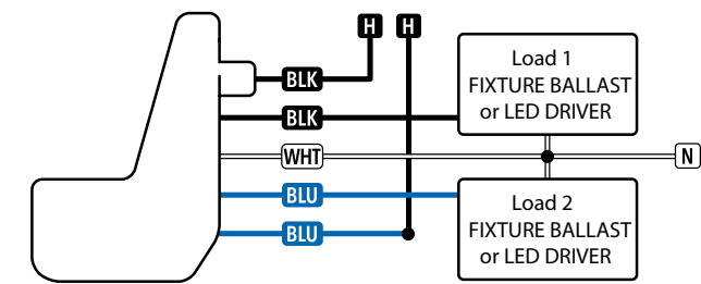
LINE VOLTAGE INTERCHANGEABLE LENS FIXTURE MOUNT: 2-POLE SWITCHING 120/277 VAC (MVOLT)
