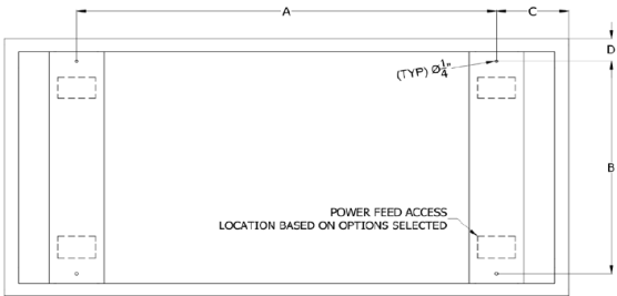
Surface mount dimensions
